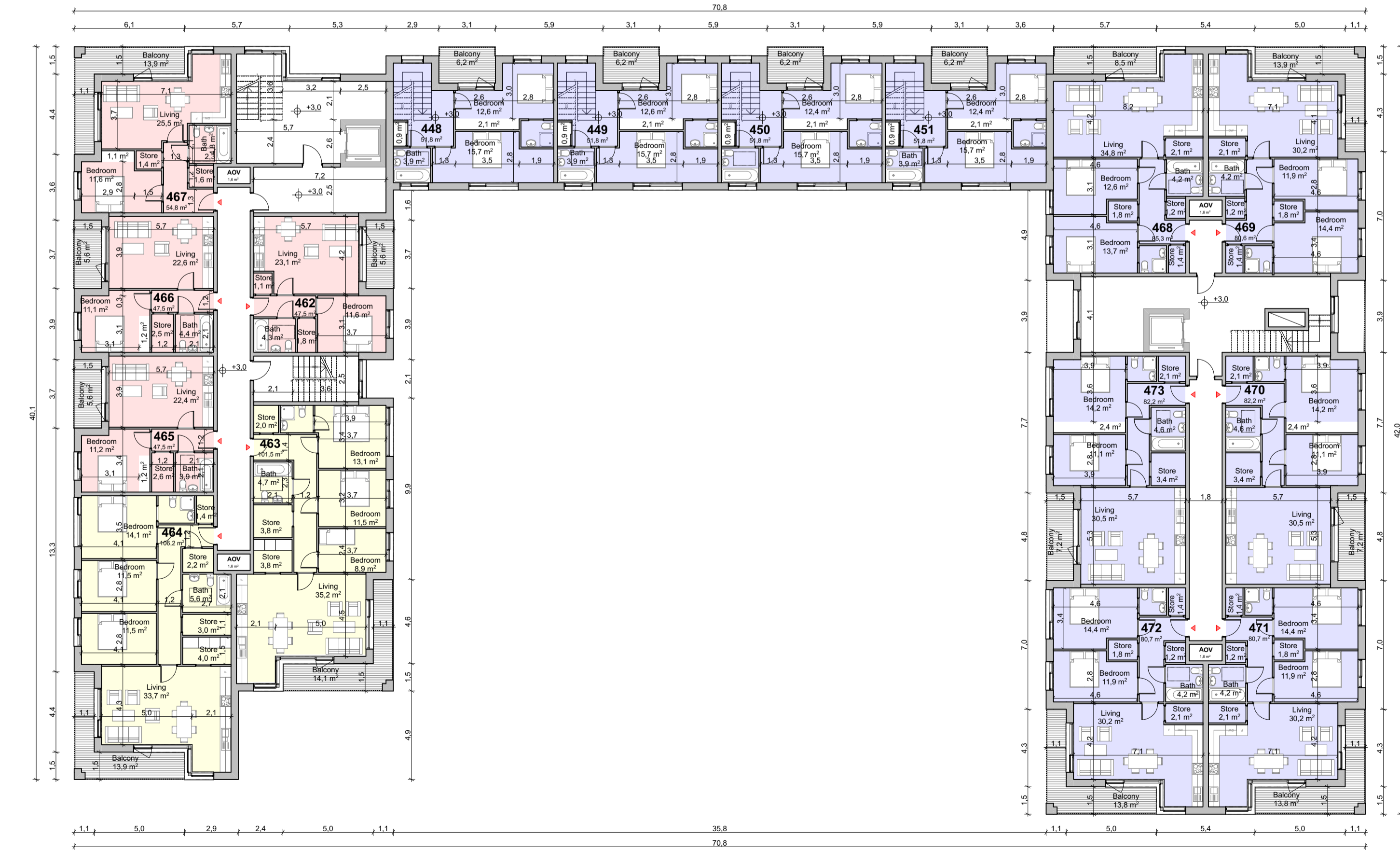
First Floor Plan 1:200
